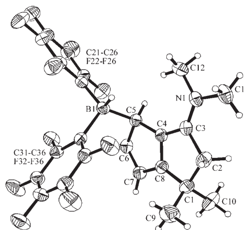
Figure 2. Molecular structure of the kinetic HB(C 6 F 5 ) 2 addition product 7a .
