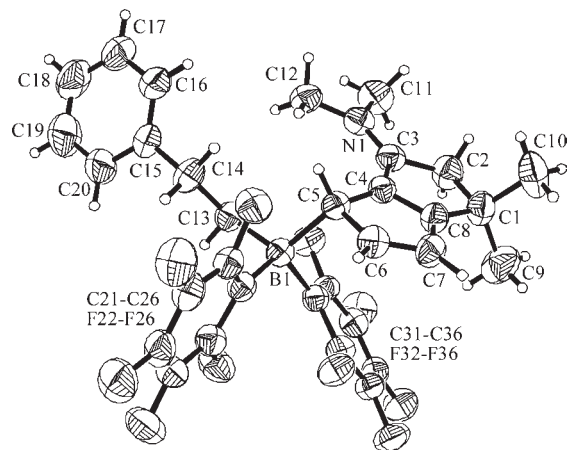
Figure 7. Molecular structure of 11 .
