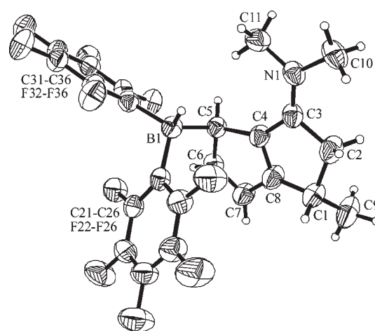
Figure 4. Molecular structure of anti - 7b .
