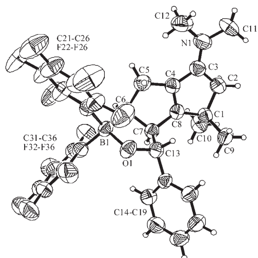
Figure 9. Molecular structure of 14 (molecule A is shown).
