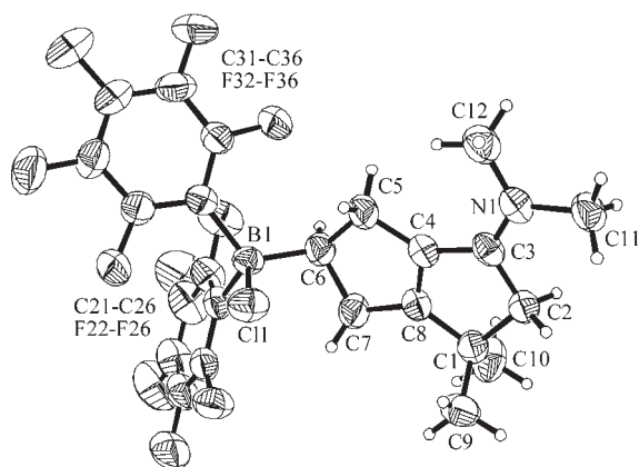
Figure 8. Molecular structure of 13.
