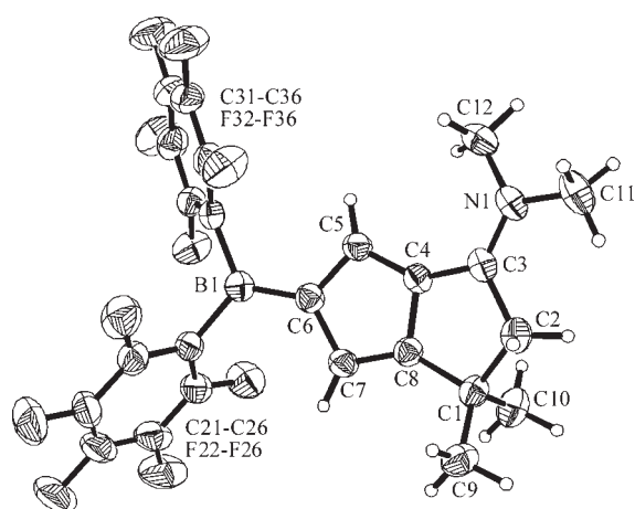
Figure 3. Molecular structure of 10a .
