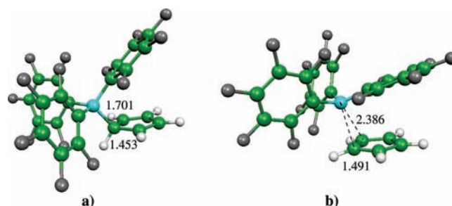
Figure 6. Optimized structures (TPSS-D3/def2-TZVP) of the minimum (a) and TS (b) for R = B(C 6 F 5 ) 3 . The bond lengths are given in angstroms.
