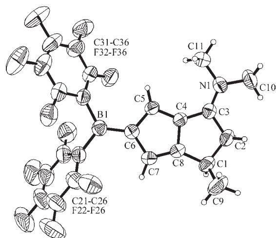
Figure 5. Molecular structure of 10b.
