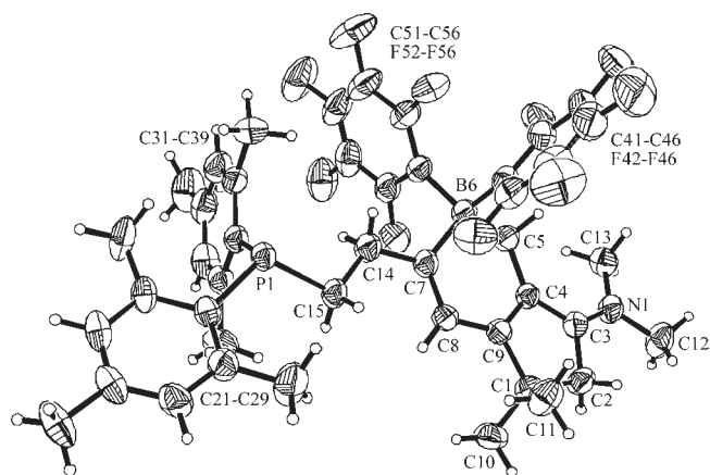
Figure 1. Projection of the molecular geometry of the ring-expanded product 3c . Selected bond lengths (Å) and angles (deg): C3–N1 1.320(3), C3–C4 1.427(3), C4–C9 1.373(3), C8–C9 1.436(3), C7–C8 1.344(3), C7–B6 1.631(3), C5–B6 1.657(3), C5–B6–C7 109.8(2), C8–C7–B6 121.1(2), C4–C5–B6 112.5(2).
